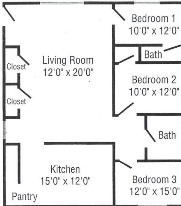
Typical Three Bedroom
